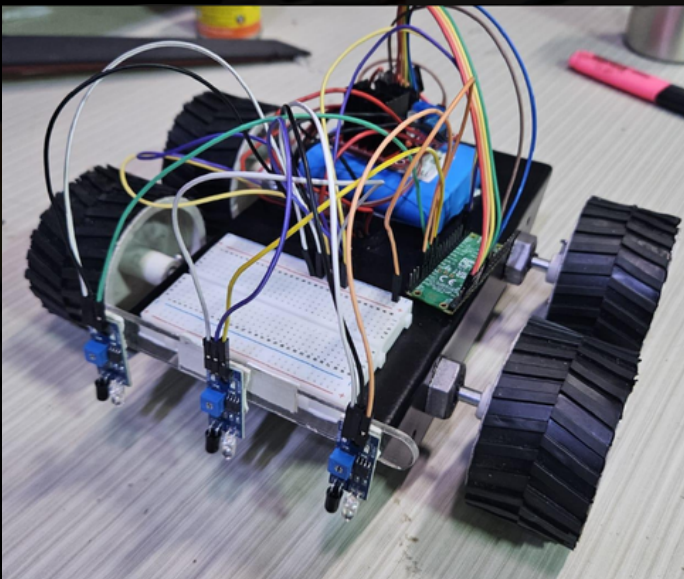
LINE FOLLOWER
